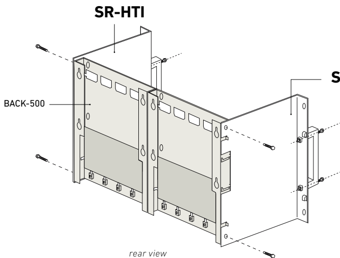
Rack 19" fixing for two base-plates (BACK-500) headend installation
